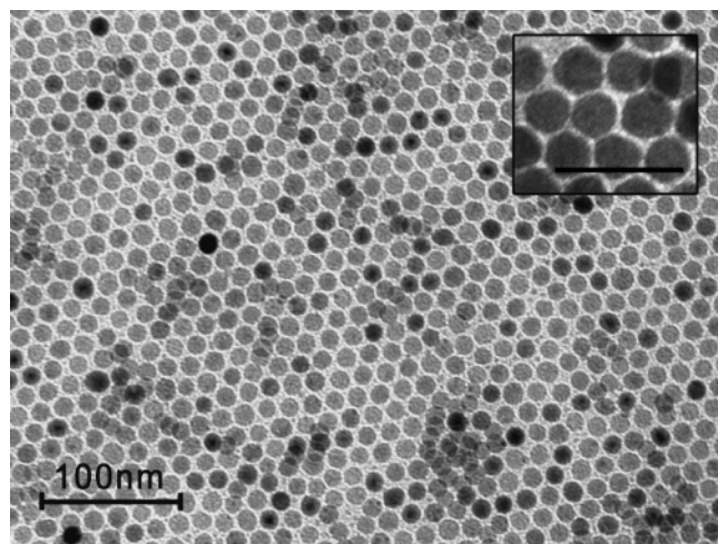
Figure 1. TEM image of iron oxide nanocrystals obtained by using \text{Fe}(\text{CO})_5 :mCPBA = 1:1.5. Scale bar in the inset is 50 nm.
