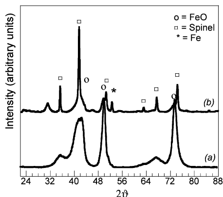
Figure 6. XRD spectra of the nanocrystals obtained by using \text{Fe}(\text{CO})_5 :mCPBA = 1:1.5 after a growth time of 5 min (a) and 1 h 30 min (b). The radiation used is Co K\alpha .
