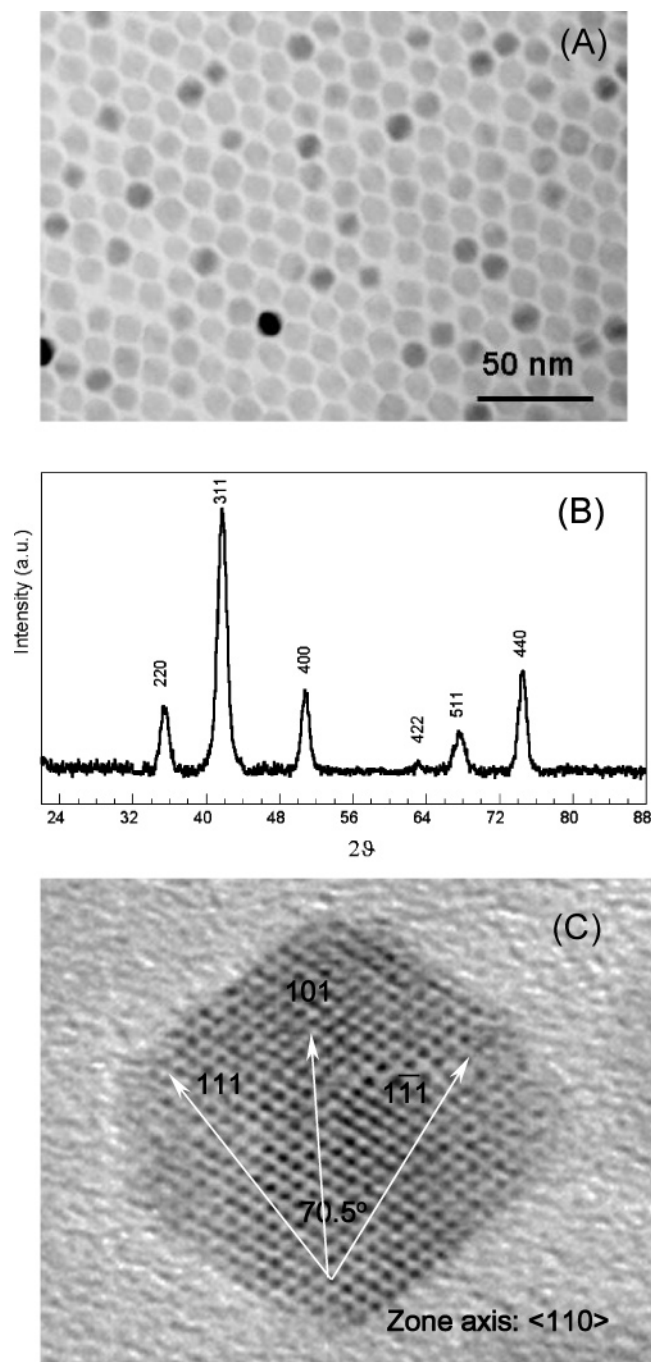
Figure 5. Low-resolution TEM image (A), XRD spectrum (B), and high-resolution TEM (C) of the sample obtained by performing sequential injections of oxidizer to obtain single-crystalline spinel nanocrystals.
