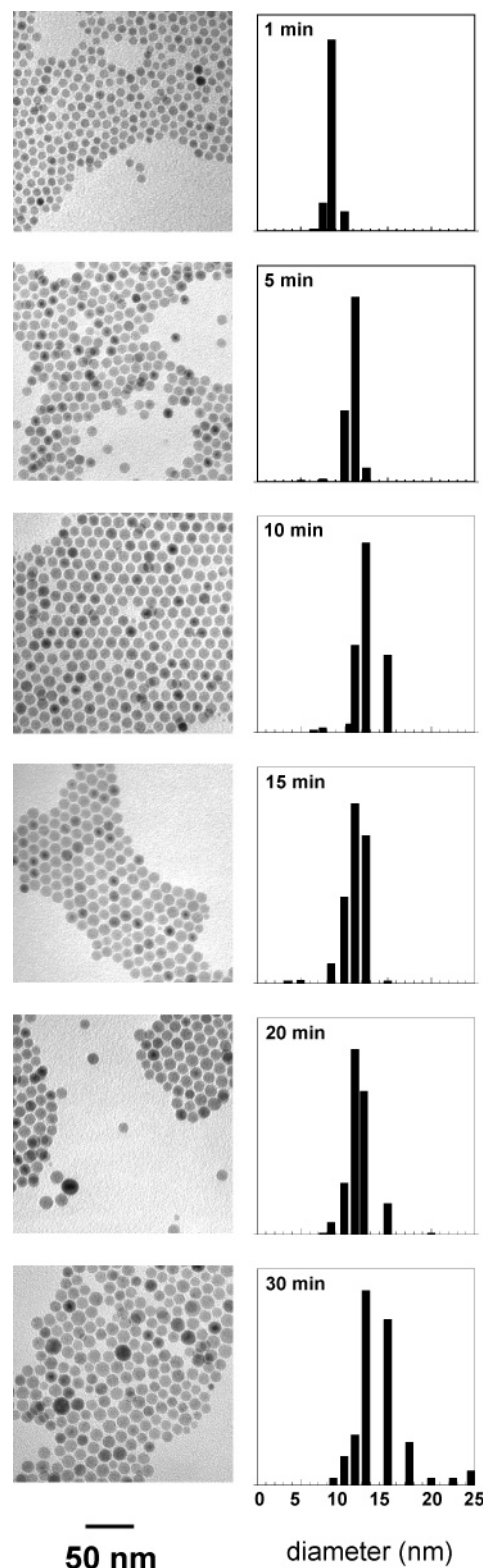
Figure 2. TEM images (left) and size distributions (right) obtained by using \text{Fe}(\text{CO})_5 :mCPBA = 1:1.5 at increasing growth time.
