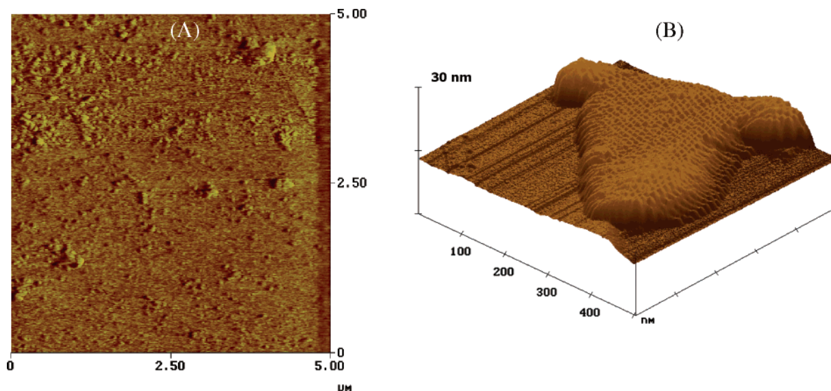
Figure 3. AFM image of iron oxide nanocrystals obtained by using \text{Fe}(\text{CO})_5 :mCPBA = 1:1.5, isolated particles (A), and a 3D representation of an AFM image of a self-assembled multilayer (B).
