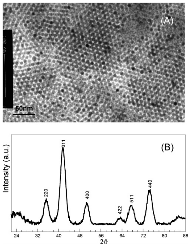
Figure 7. Low-resolution TEM image (A) and XRD spectrum (B) of the sample obtained by carrying the synthesis at higher temperature followed by a second injection of oxidizer.
