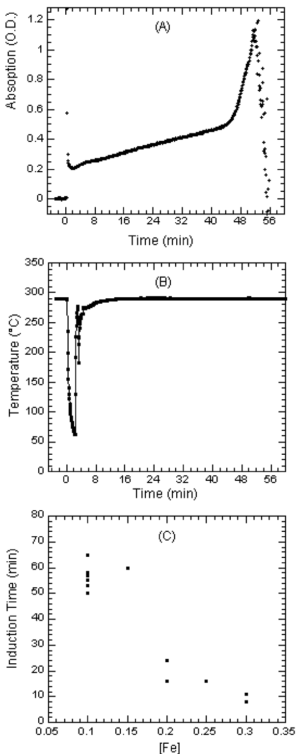
Figure 4. Optical density of the solution collected in situ at 440 nm during a typical synthesis carried out with molar ratios of \text{Fe}(\text{CO})_5 :mCPBA = 1:1.5 (A) and corresponding temperature variation (B). The time = 0 corresponds to the injection time; the induction time for particle formation under these conditions is about 1 h. The dependence of the induction time on the iron precursor molar concentration is reported in (C).
